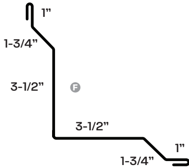
413 Inside Corner
