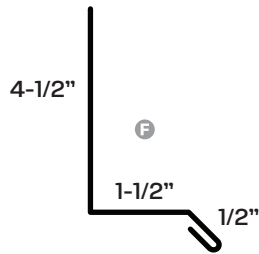
499 Drip Cap
