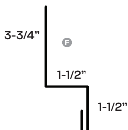
407 Gable Divider
