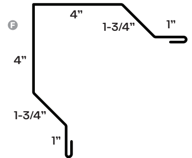
494 Outside Corner
