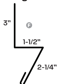
461 Angle Base
