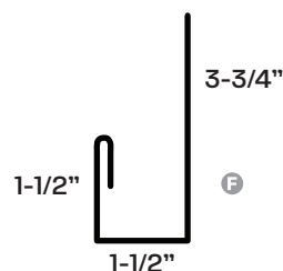
492 J-Channel
