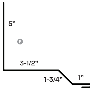
400 Sidewall
