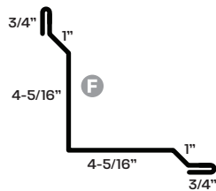
113 Inside Corner
