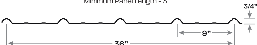
38" Manufactured Panel with 36" Finish Reveal
