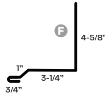
100 Sidewall
