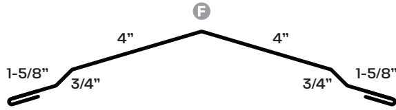
91 Ridge Cap
