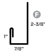
92 J-Channel
