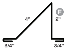
140 Pipe Guard
