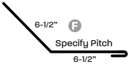
110 Endwall/Transition
