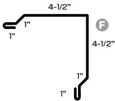
94 Large Rake/Corner
