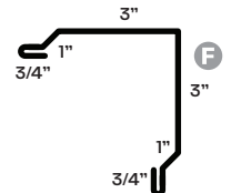
104 Rake/Corner
