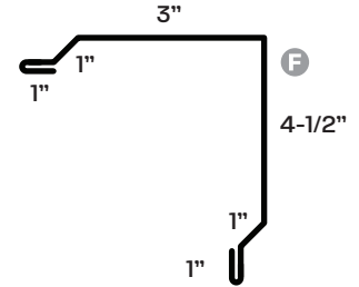
125 Offset Rake/Corner
