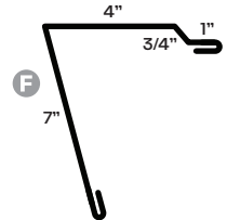
MSR Mono Slope Ridge
