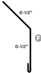
111 Gambrel Transition
