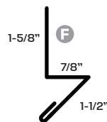
161 Angled Base
