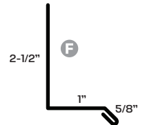
199 Drip Cap
