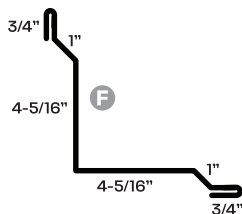
MSR Mono Slope Ridge
