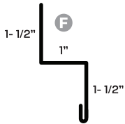
107 Gable Divider
