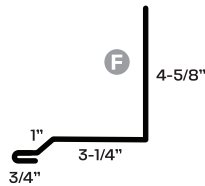
100 Sidewall
