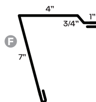
MSR Mono Slope Ridge
