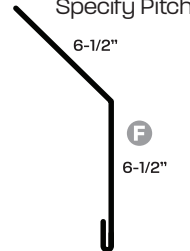
161 Angled Base
