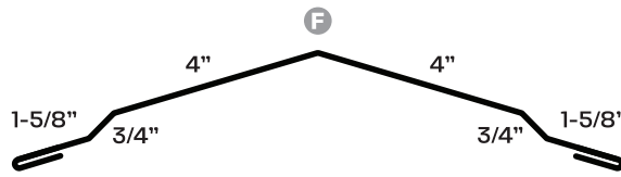
91 Ridge Cap
