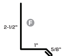
199 Drip Cap
