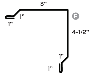
125 Offset Rake/Corner
