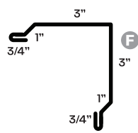
104 Rake/Corner
