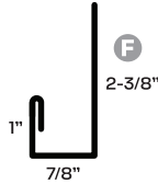
92 J-Channel
