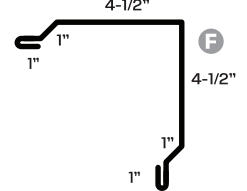
140 Pipe Guard
